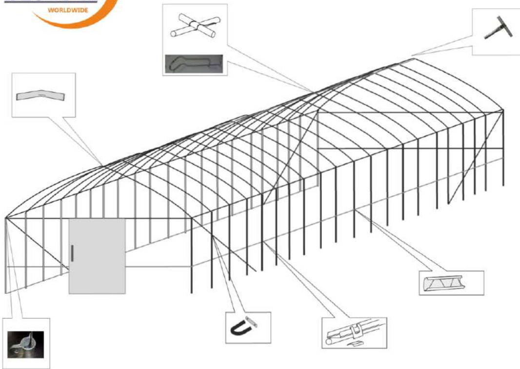
C-PROFILE WITH ZIG-ZAG SPRING SYSTEM FOR SHEET FIXING
